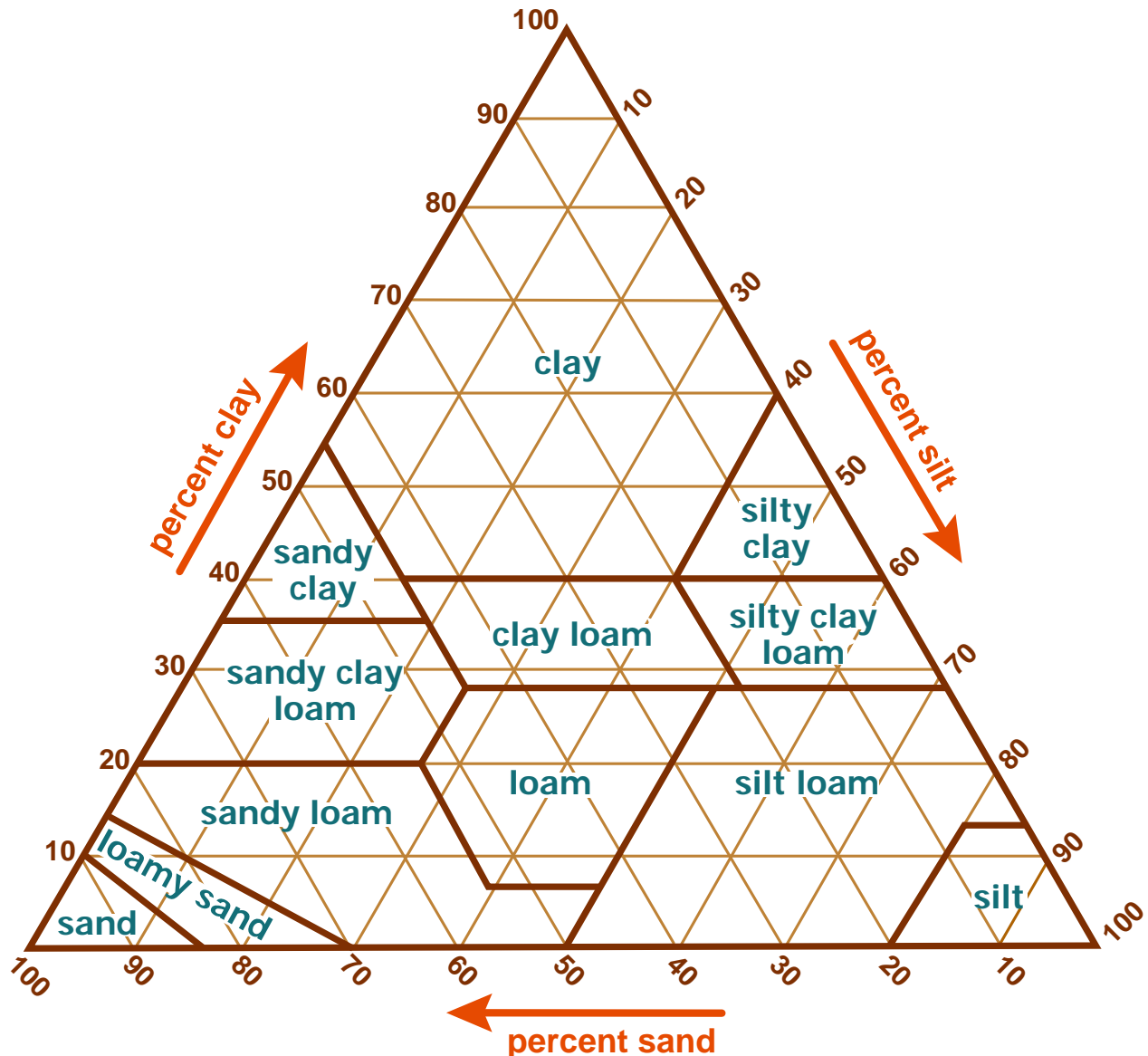
The Textural Triangle
